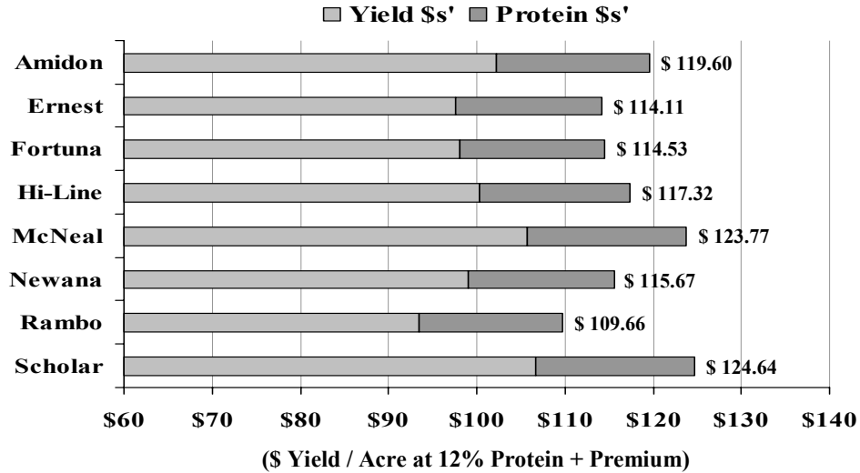
Figure 7. MSU/AES/NARC-Havre Ref=04-9907 P=.0308 CV2=2.73%
