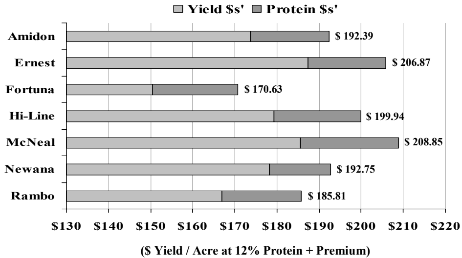
Figure 5. MSU/AES/NARC-Havre Ref=04-9921 P=.0001 CV2=2.69%
