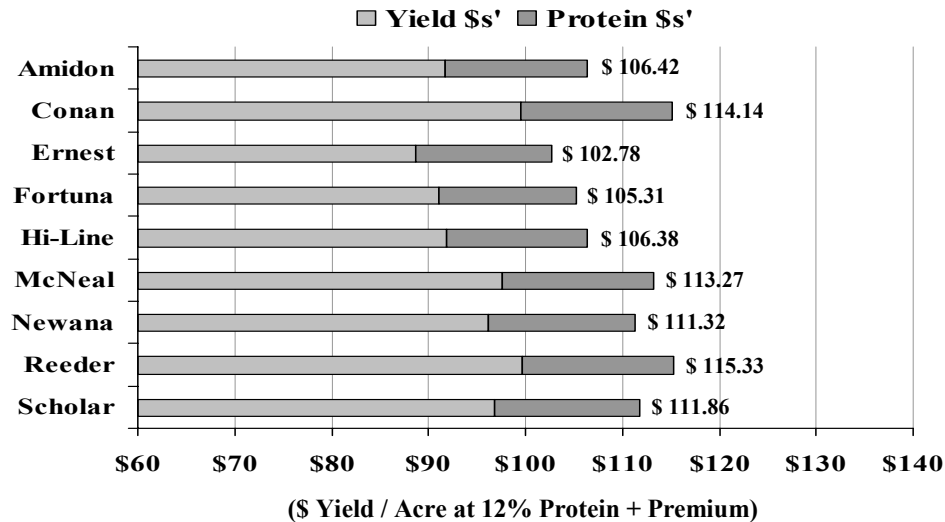
Figure 7a. MSU/AES/NARC-Havre Ref=04-9917 P=.4279 CV2=4.02%
