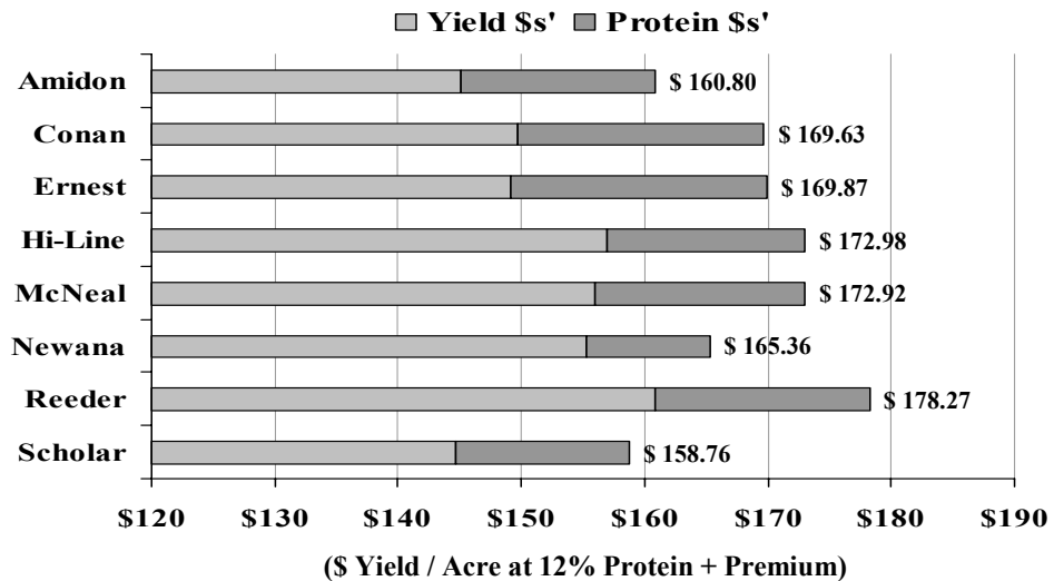
Figure 6a. MSU/AES/NARC-Havre Ref=04-9915 P=.0330 CV2=2.46%
