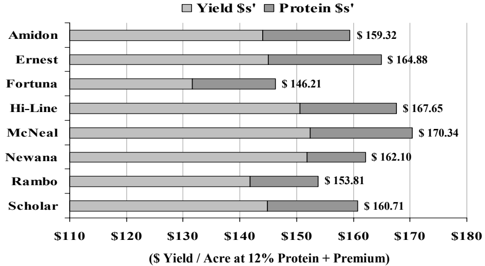
Figure 6. MSU/AES/NARC-Havre Ref=04-9905 P=.0011 CV2=2.39%
