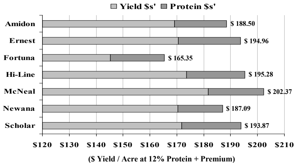
Figure 5a. MSU/AES/NARC-Havre Ref=04-9941 P=.0001 CV2=2.10%
