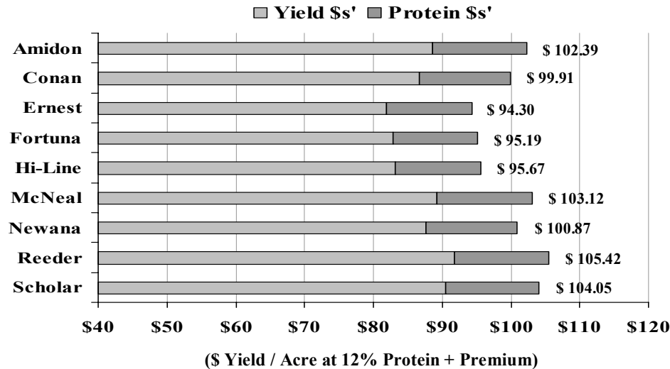
Figure 7a. MSU/AES/NARC-Havre Ref=03-9917 P=.4908 CV2=4.23%
